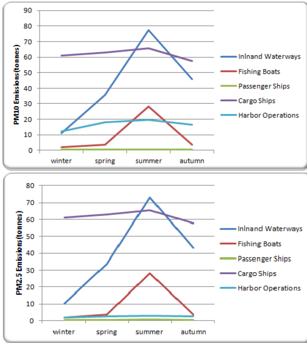
Figure 2.3.: Seasonal variability of a) PM10 and b) PM2.5 emissions for each maritime activity (reference year 2020).
