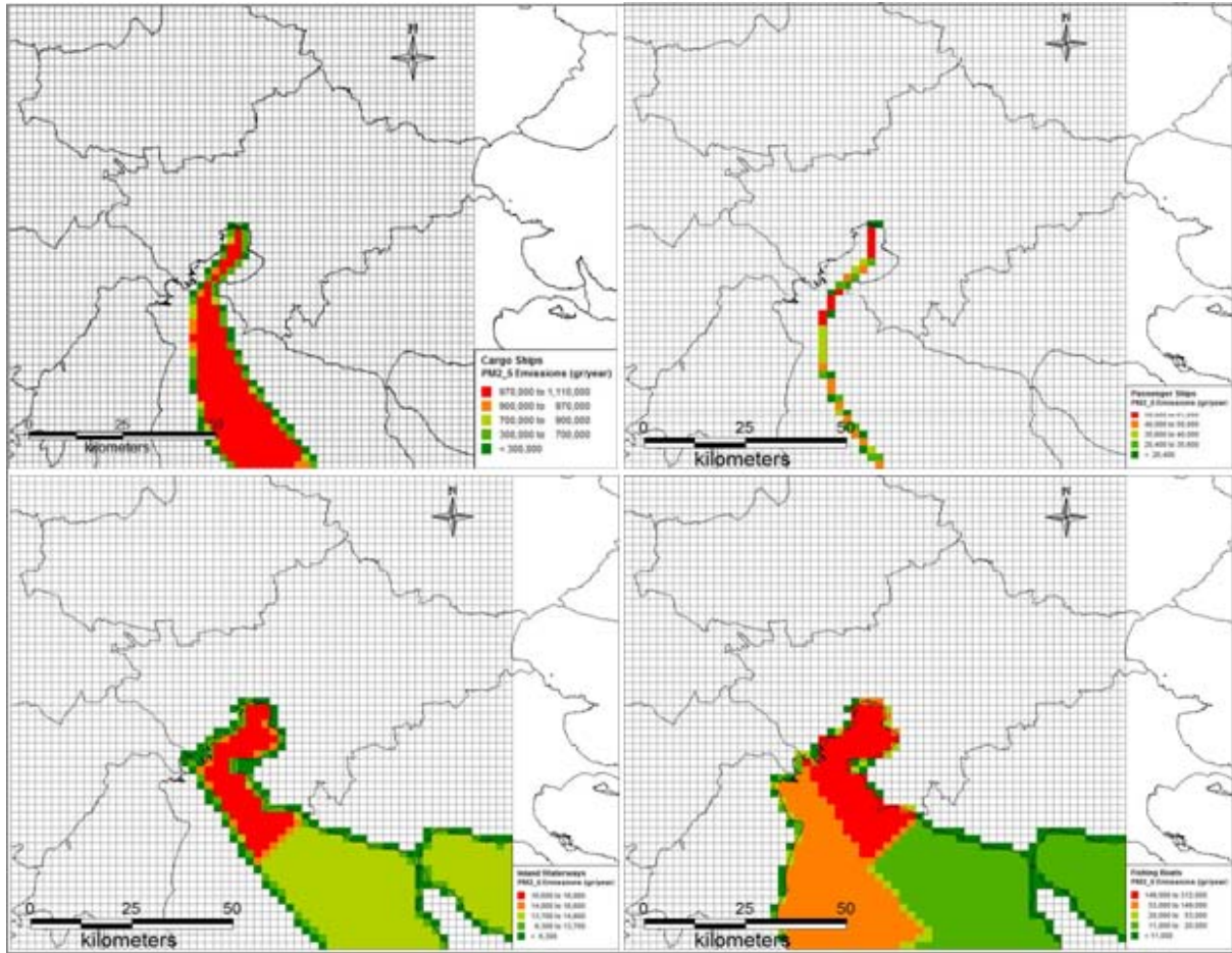
Figure 1.3: Annual PM2.5 emissions from cargo ships, passenger ships, inland waterways and fishing boats (ship emissions presented for all transport modes: on-route, maneuvering and hotelling) (reference year 2010).
