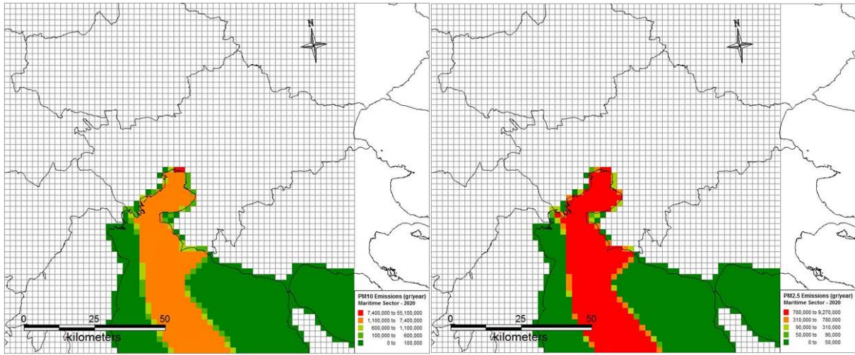
Figure 2.2.: Annual PM10 and PM2.5 emissions for the maritime sector (reference year 2020).
