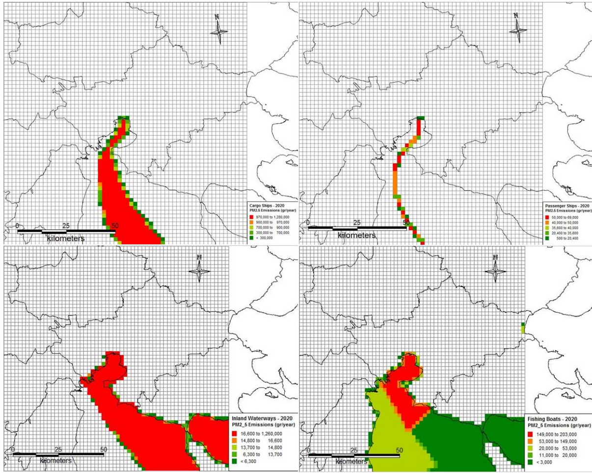
Figure 2.1: Annual PM2.5 emissions from cargo ships, passenger ships, inland waterways and fishing boats (ship emissions presented for all transport modes: on-route, maneuvering and hotelling) (reference year 2020).
