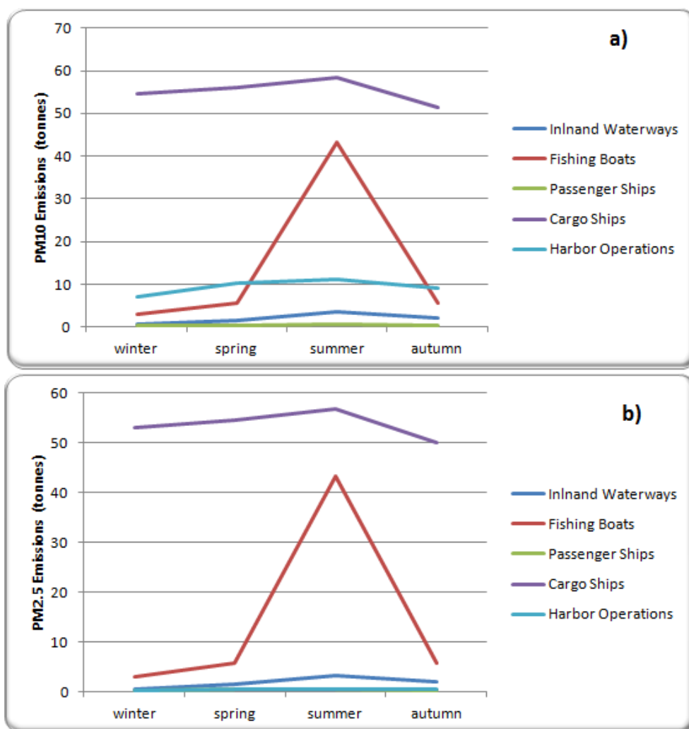
Figure 1.5.: Seasonal variability of a) PM10 and b) PM2.5 emissions for each maritime activity (reference year 2010).
